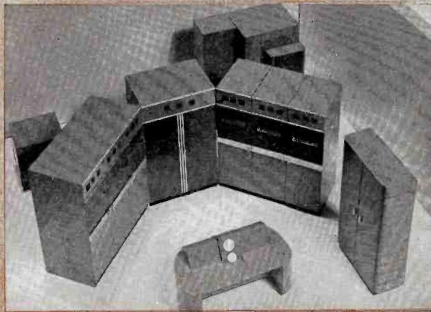
U-shaped Arrangement —several versions possible down to a minimum width of 150 inches. Transmitting equipment also includes console; sideband filter, diplexer, and dummy load (three units at right, rear); water-cooling equipment (left, rear); and racks for test and other equipment (right, foreground).
